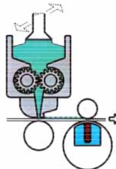
Knife-over-roll (e.g. Variopress®) with subsequent crushing
