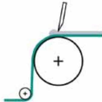
Knife-over-roll
