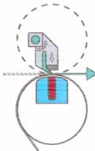
Knife (e.g. Magnetojet®) in a rotary screen
