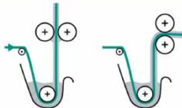
Foulard with horizontal/vertical squeezing rollers
