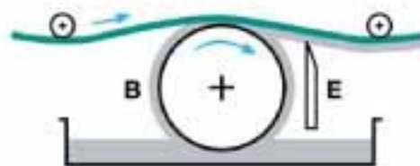
Application Roller/ Kiss Coater
